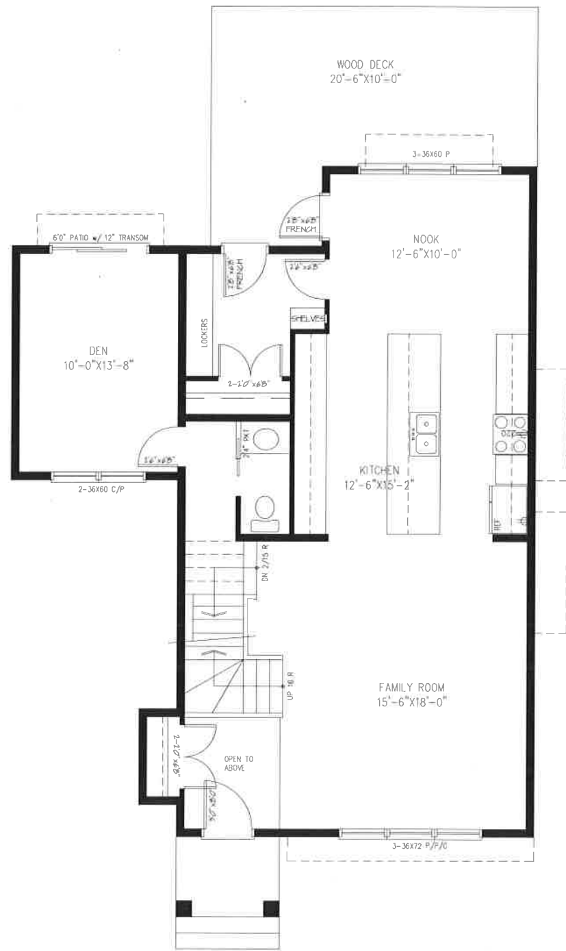
MAIN FLOOR AREA : 1068 SQ. FT TOTAL AREA : 2086 SQ. FT 9'-1" CEILING HEIGHT TOP OF WINDOWS @ 8'-0"
