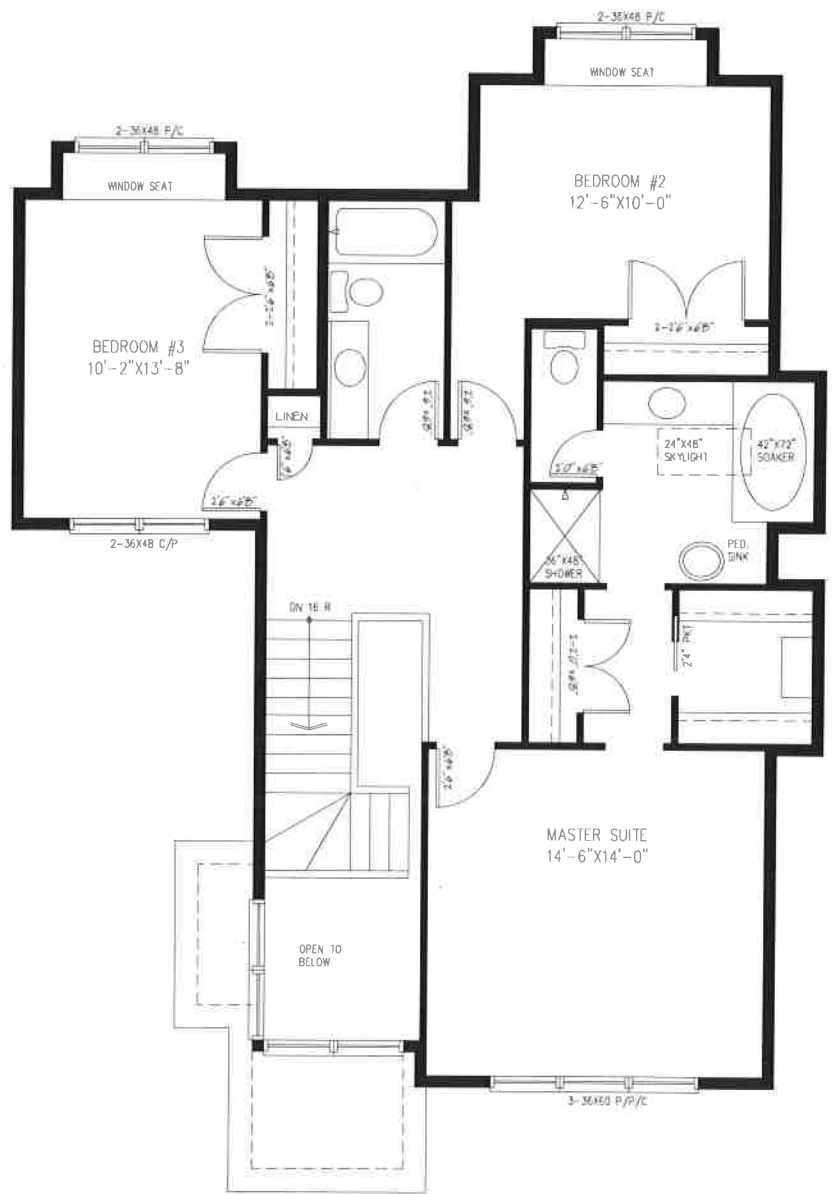
SECOND FLOOR AREA : 1018 SQ. FT 8'-1" CEILING HEIGHT TOP OF WINDOWS @ 7'-0"
